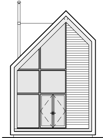
2/3 Glazing Wall (Swing Door)
